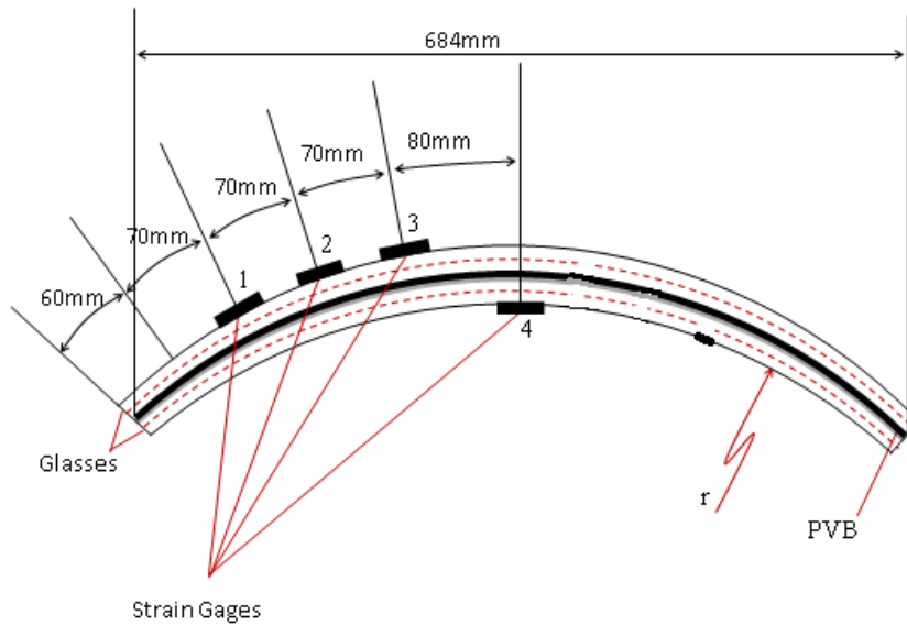
Figure 2. Curved laminated glass beam sample
