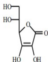
Vitamin C
