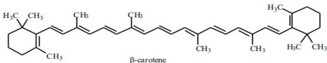
β-carotene
