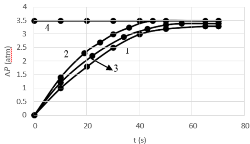
Fig. 3. Pressure Recovery Curves. 1-pure water, 2- water with 0.006% additive, 3- water with 0.045% additive, 4-inlet pressure of the model
