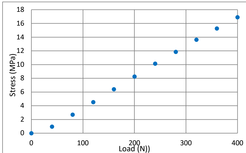
Figure 8. Stress values from the strain gage 1
