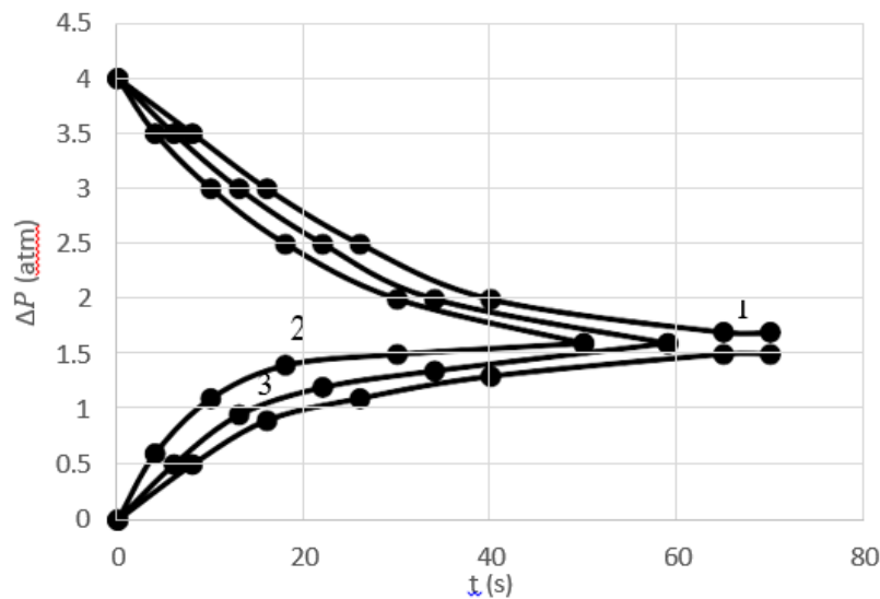
Fig. 4. Pressure Recovery Curves. 1-pure water, 2- water with 0.006% additive, 3- water with 0.045% additive
