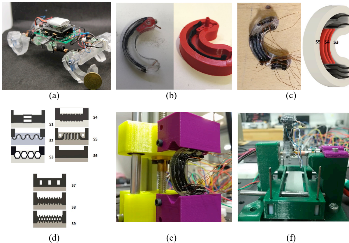
Figure 1. Development and testing of the soft sensor presented by Ozbek et al. (a) C-legged Squad robot, (b) C-shaped flexible structure containing a single resistive sensor and the mould obtained from the 3D printer used in sensor production, (c) C-shaped flexible sensor structure consisting of 8 flexible resistive sensors and the placement of resistive sensors labelled with S1-S8 in the C structure, (d) various sensor geometries tested, (e) the force test for the sensor placement and (f) the treadmill test for speed measurement
