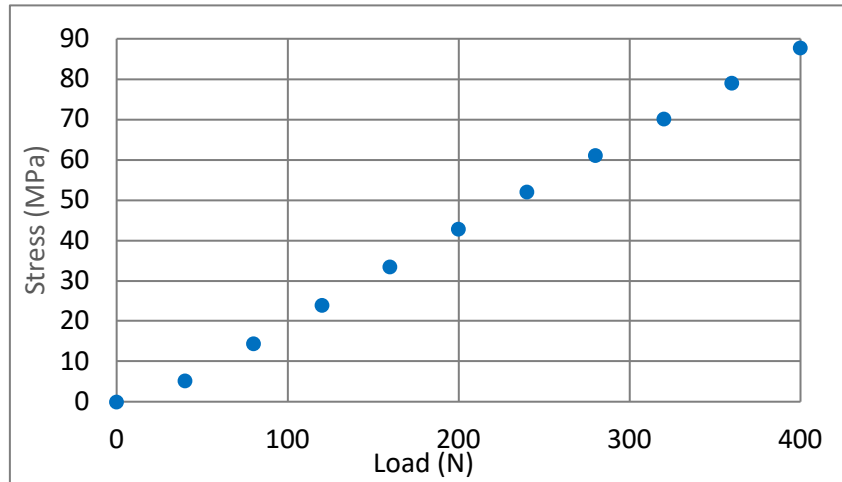
Figure 7. Maximum stress values from the strain gage 4 at the center
