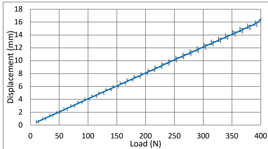
Figure 6. Central displacement values from the material testing machine
