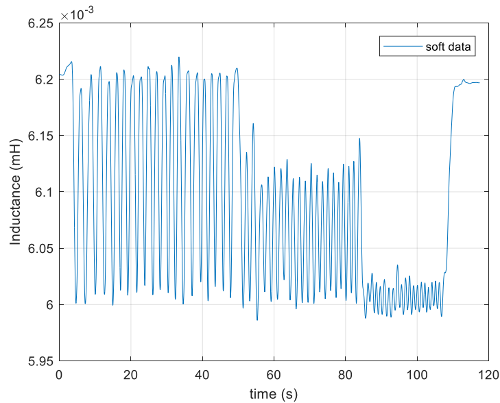
Figure. 4. Electrical response of the developed soft sensor
