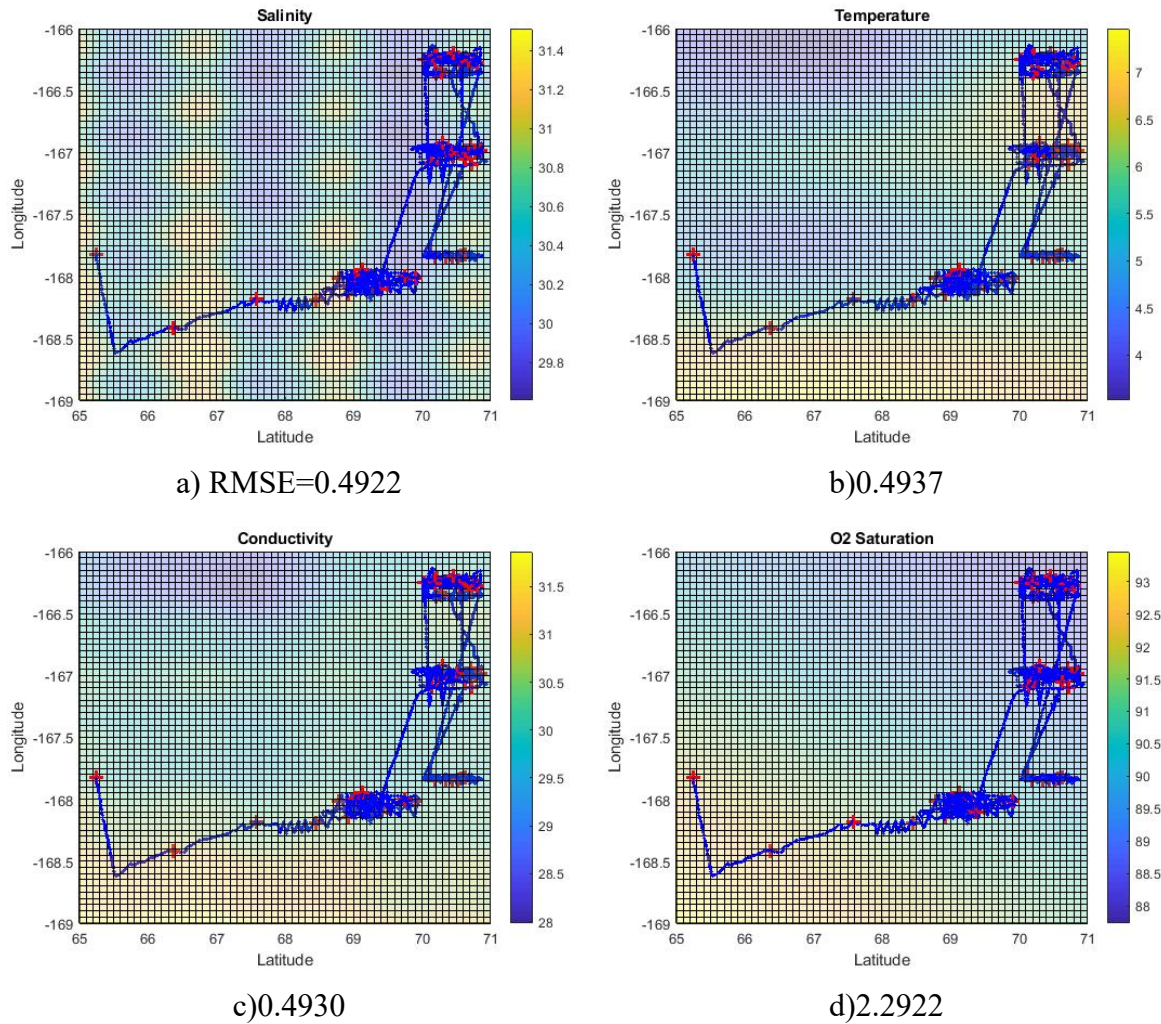
Figure 1. The estimated WQI parameters a) Salinity b) Temperature c) Conductivity d) O 2 Saturation
