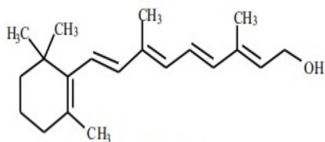
Vitamin A
