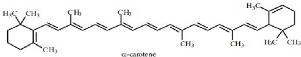
α-carotene
