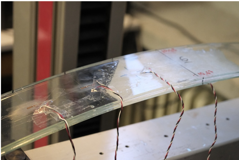
Figure 4. Location of strain gages on curved laminated glass beam
