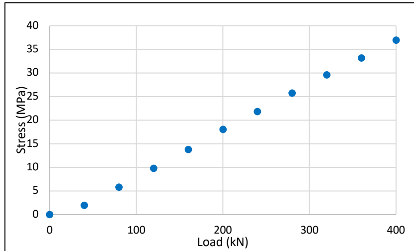
Figure 9. Stress values from the strain gage 2
