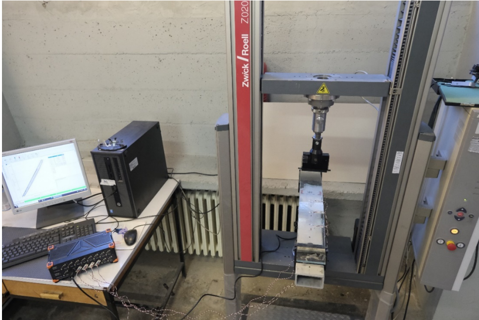
Figure 5. Experimental setup
