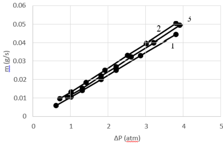
Fig. 2. Mass flow curves. 1-pure water, 2- water with 0.006% additive, 3- water with 0.045% additive
