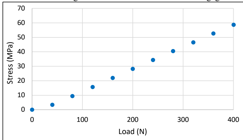
Figure 10. Stress values from the strain gage 3
